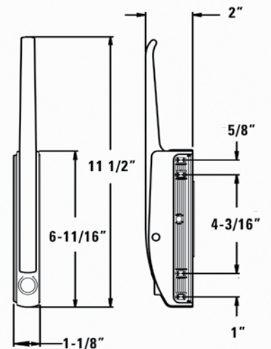
171 STRAIGHT DIE-CAST OR COMPOSITE HANDLE
